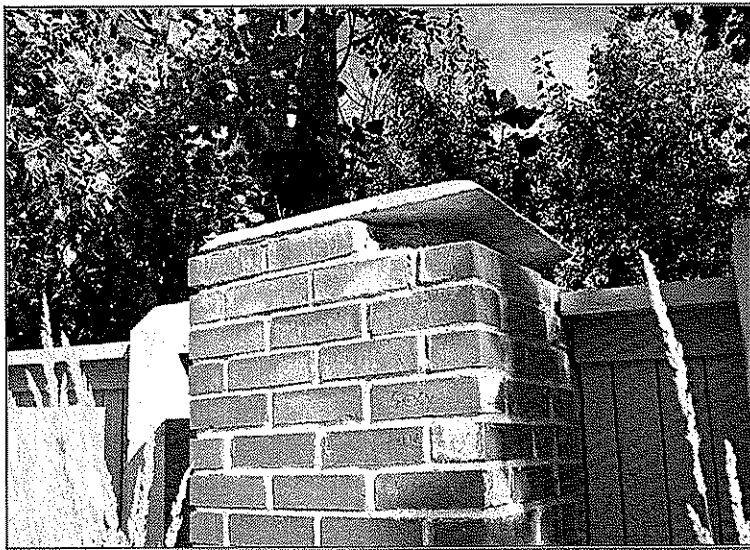
Bricks missing and mortar deterioration at the Himalaya Street pillars
