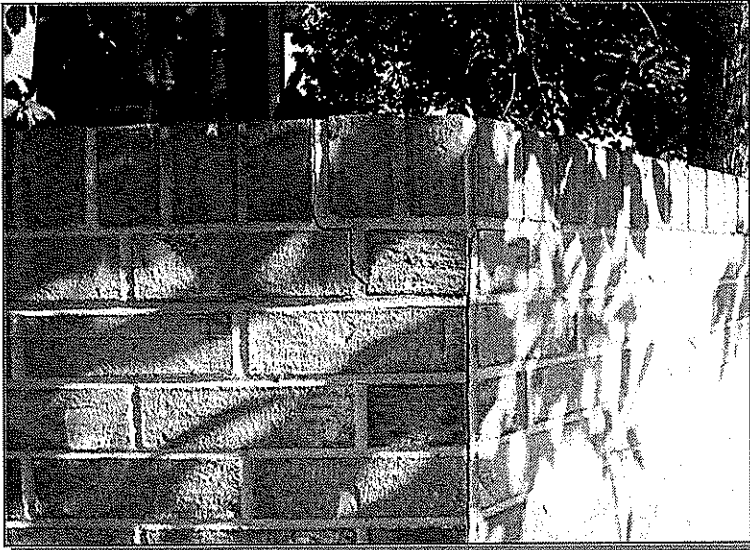
Cracks in the monument wall at Genoa Street
